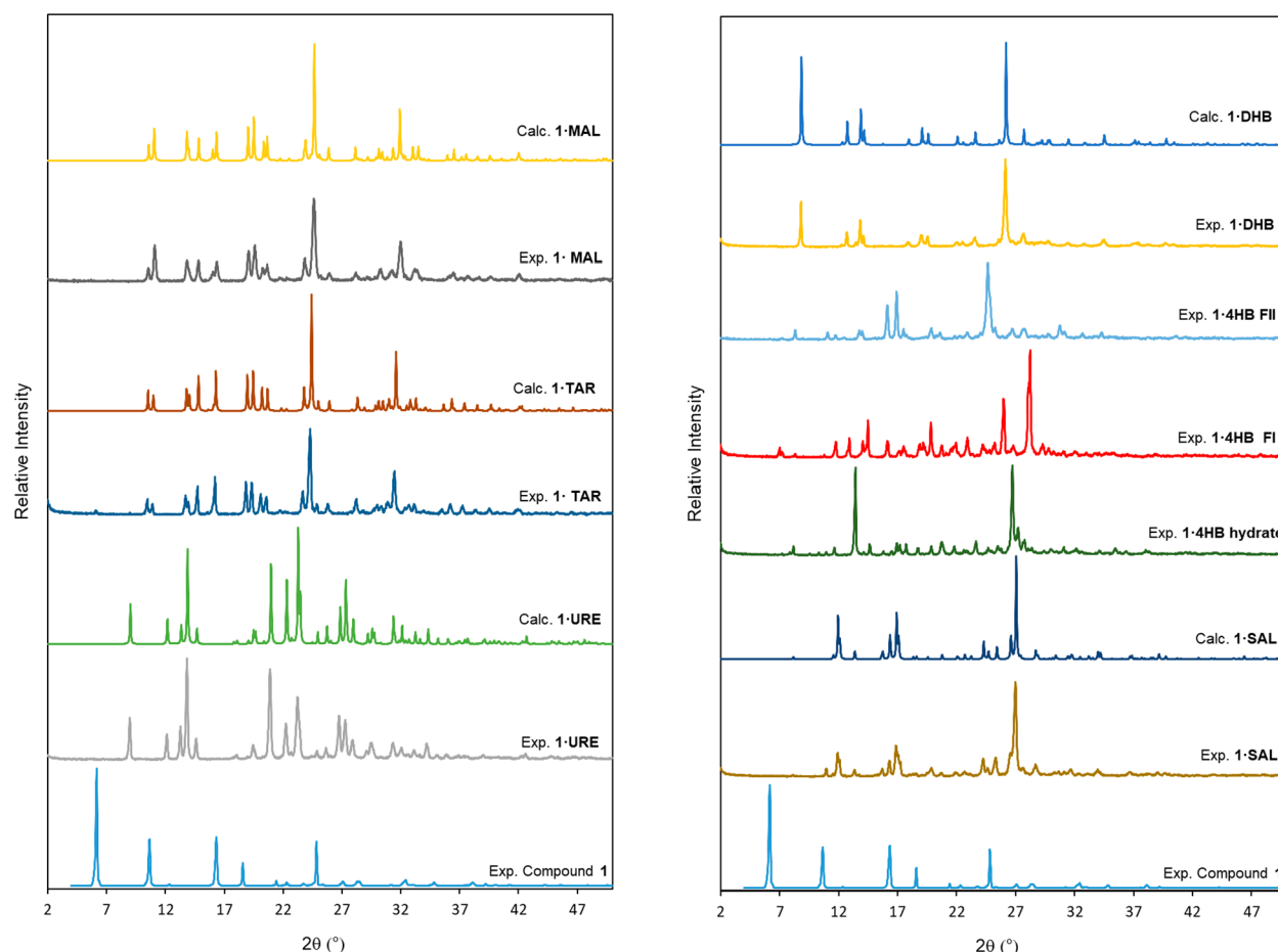
Figure 1. Comparison of the experimental and calculated PXRD patterns of 1 and the as-synthesized cocrystals 1 · URE , 1 · TAR , 1 · MAL , 1 · SAL , 1 · 4HB · H 2 O , 1 · 4HB _FI, 1 · 4HB _FII, and 1 · DHB .
